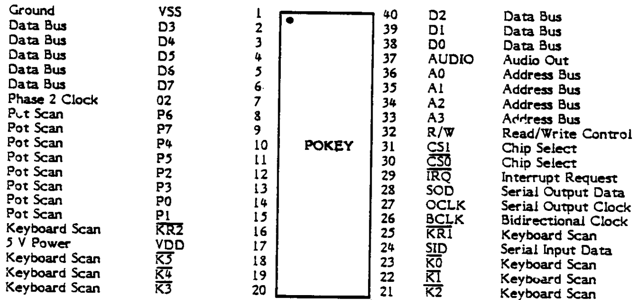
Figure 1-6. POKEY Pin Assignments
