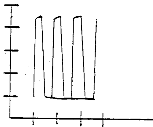
Scope Waveform 4 IuS/DIV IV/DIV
